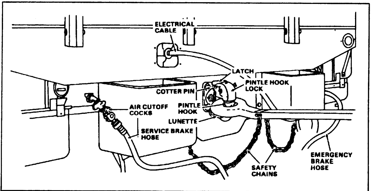
FIGURE 18-8. Vehicle and Trailer Attachment Point.
