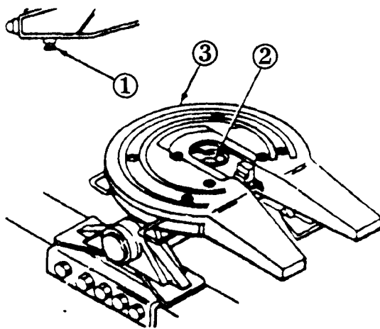
FIGURE 18-2. Coupling.
