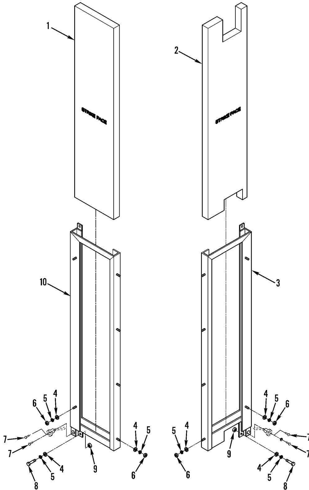
Figure 5. B-Pillar Armor
