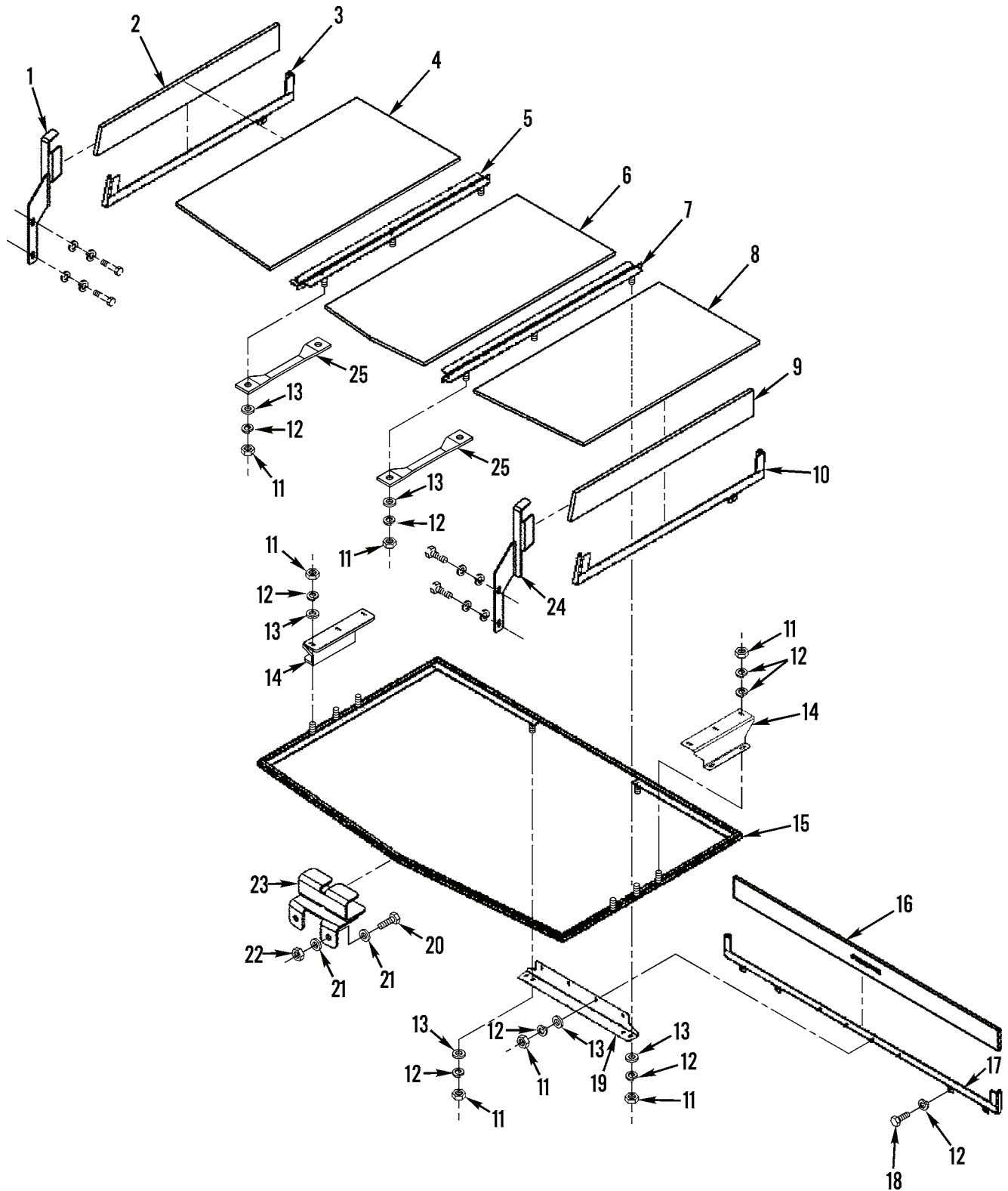
Figure 9. Roof Armor
