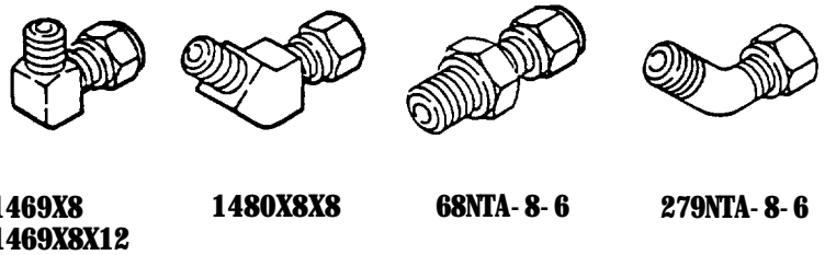
Figure E-3. 1/2" NONMETALLIC TUBING AND FITTINGS.
