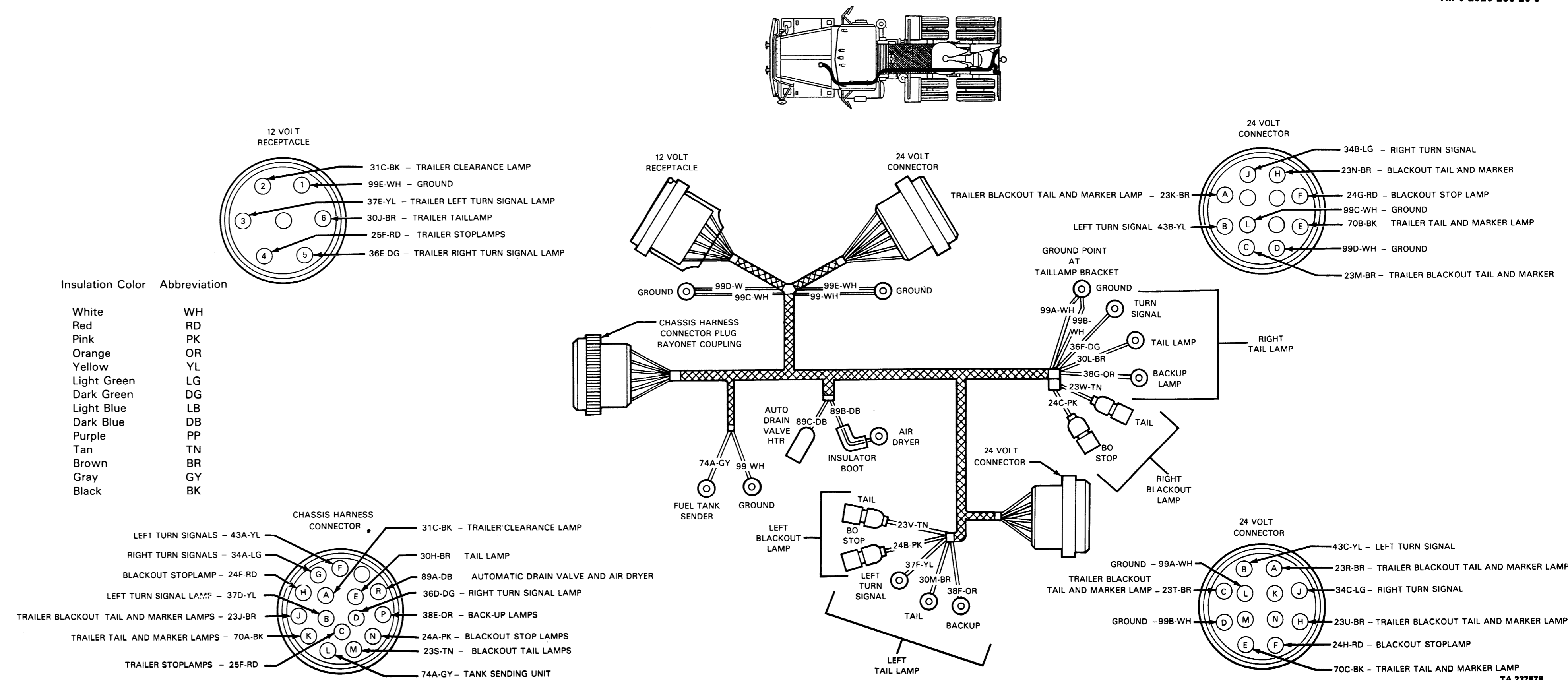
Figure FO-11. Chassis Harness Assembly
