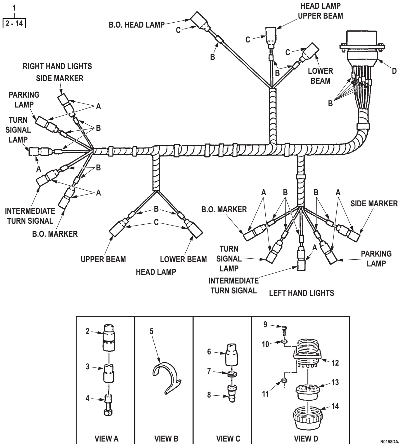
Figure 157. Harness Assembly, Front Vehicle Lights. (Sheet 1 of 2)
