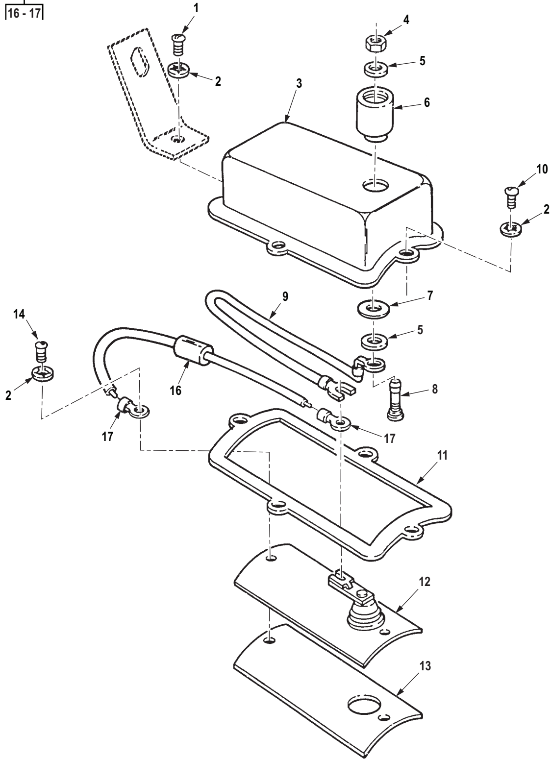
Figure 150. Horn Cover, Brush, and Capacitor Assembly.
